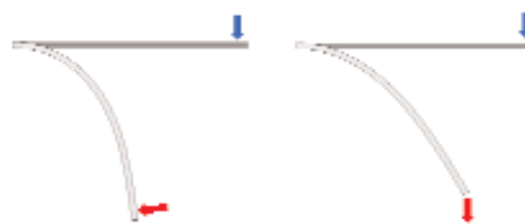
Figure 3 Following (or nonconservative) load changes its direction during the process of deformation and remains normal to the deformed beam (left). Nonfollowing, or conservative, load retains its original direction (right).
